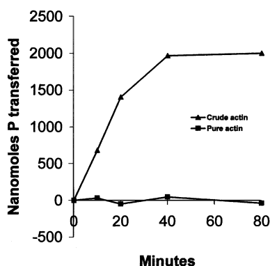
Fig. 1. Comparison of creatine kinase activity of crude and \text{Mg}^{2+} -purified actin [8,10].
